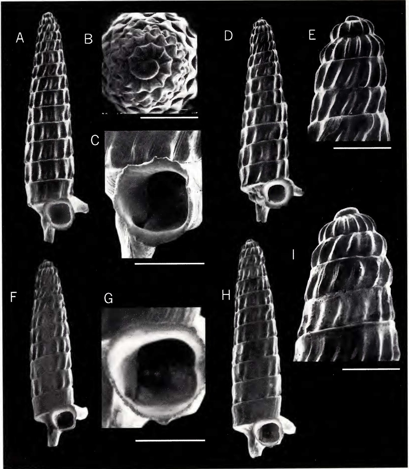
Fig. 5. Truuba anelpistos (Bouchet and Fechter, 1981). A. Shell from Meteor bank, DW152 (5.4 mm long). B. Apical view of protoconch. C. Aperture, to show the closely set edges of siphonal canal, same specimen as A. D. Shell from Hyères bank, DW188 (4.3 mm long). E. Protoconch, same specimen as D. F, H. Specimens from Irving bank, DW237 (4.2 and 5.1 mm long respectively). G. Aperture, same specimen as H. I. Protoconch, same specimen as H. Scale bars = 500 \mu m.
